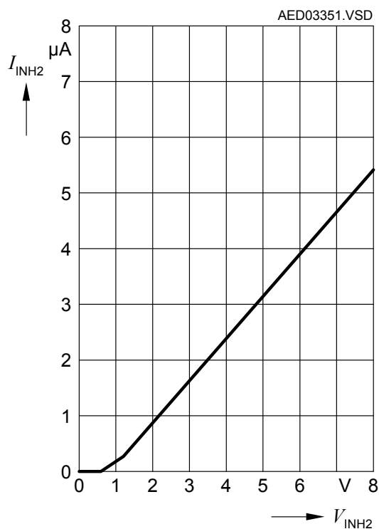
INH2 Input Current versus Inhibit Voltage
